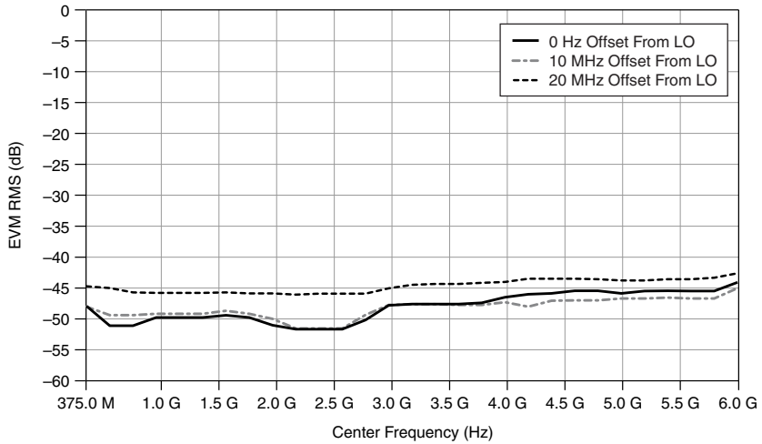
Figure 19. VSA Error Vector Magnitude, Typical 21
